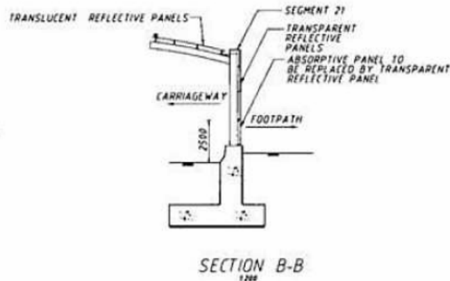
Figure 9 : Extent of the noise barrier segment nos. 20 and 21 where absorptive panels as originally provided to a height of 2.5m above the road level are replaced by transparent reflective panels
